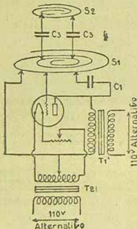
(Fig. 1) — Schema theorico
